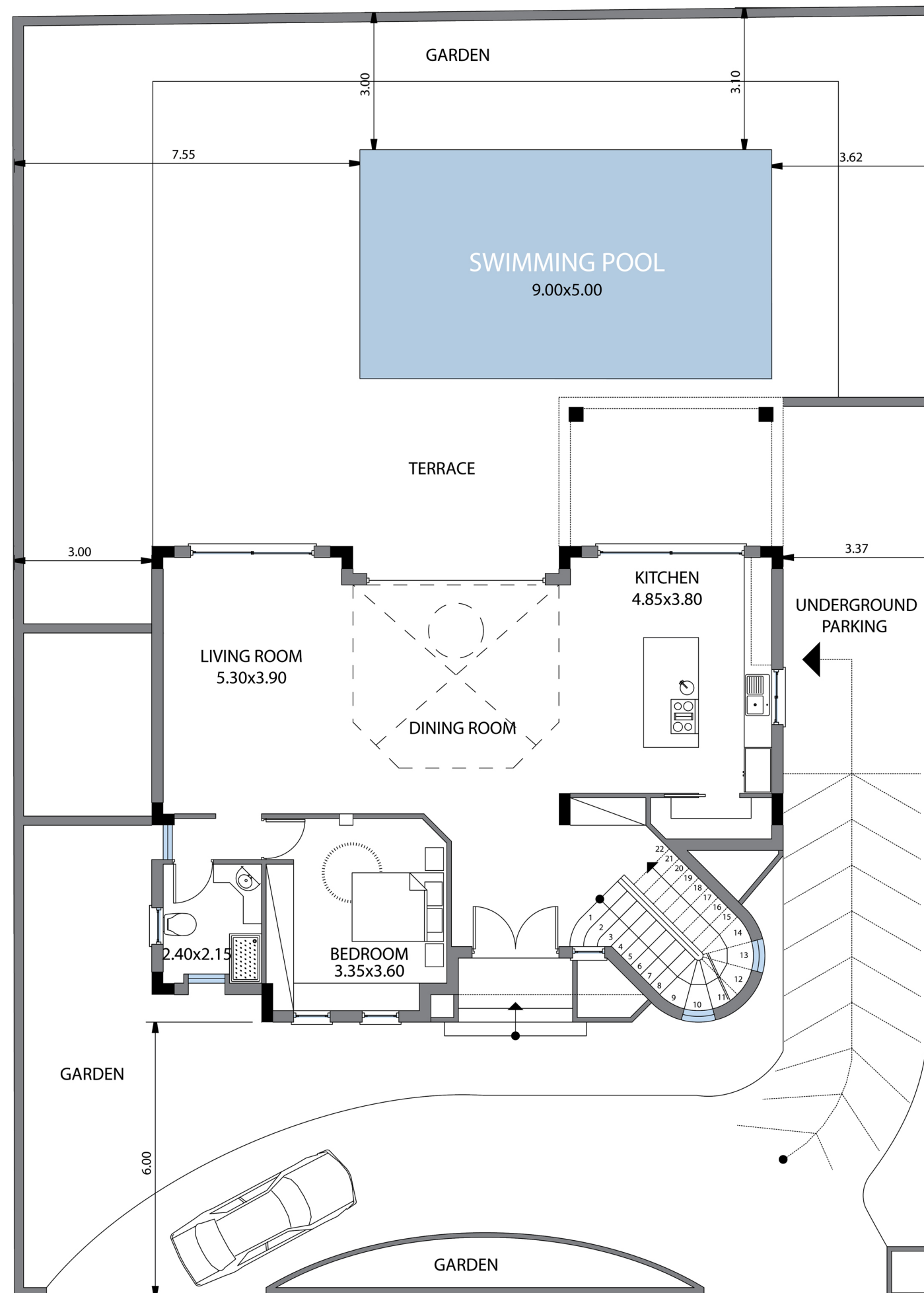
GROUND / SITE PLAN VIEW - Type B
